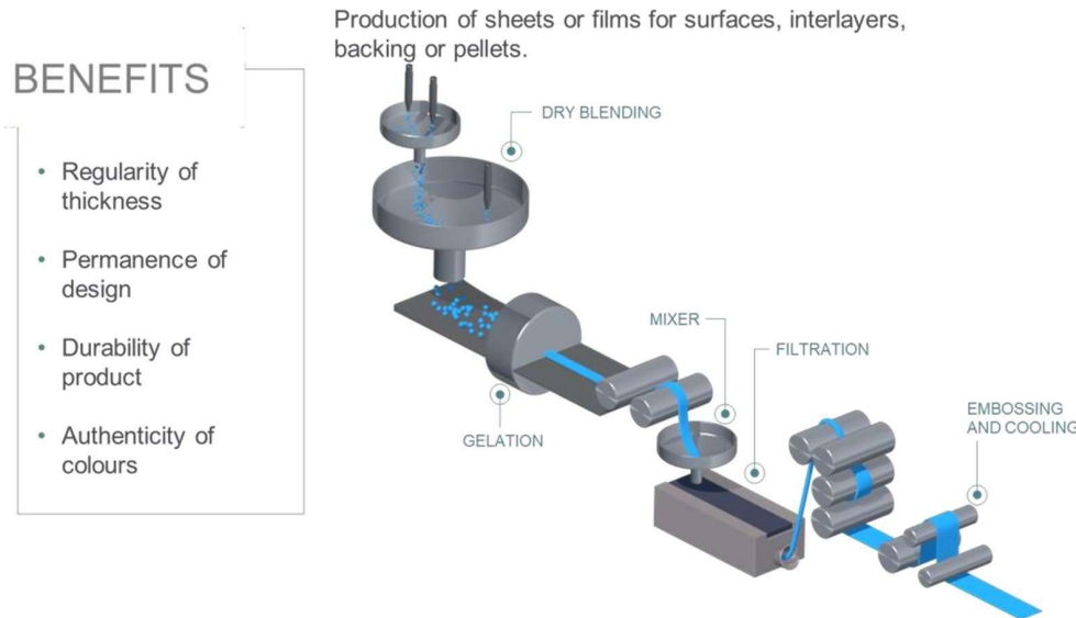
Figure 3: Calendering process
